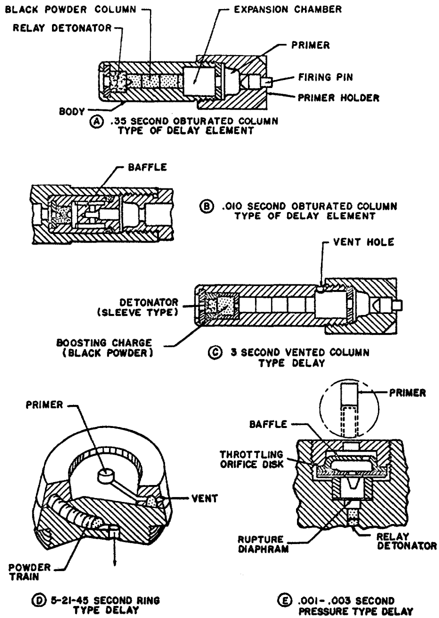
Fig 1-46 ARMY AND NAVY DELAY ELEMENTS AND DELAYS
